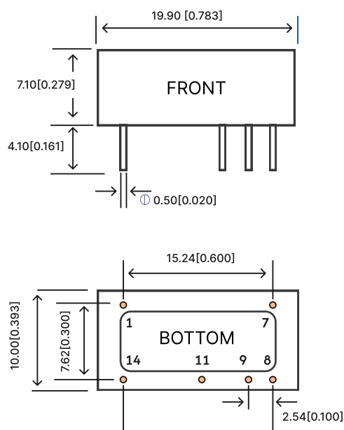
Figure 7: Overall dimensions
