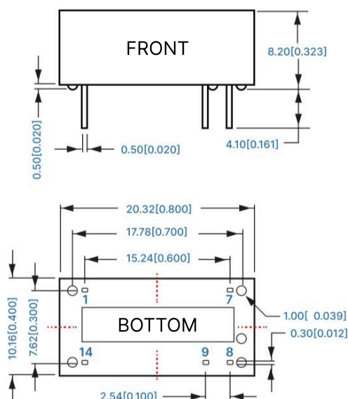
Figure 7: Overall dimensions
