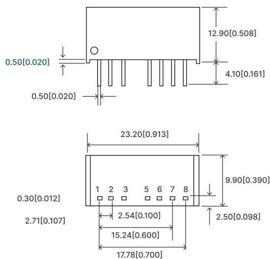
Figure 7: Overall dimensions
