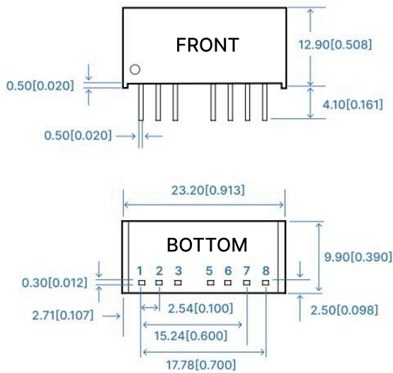
Figure 7: Overall dimensions
