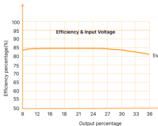
Figure 7: Efficiency Vs Input Voltage (100% Load)
