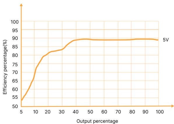
Figure 6: Efficiency Vs Output Load (Nominal Voltage Input)
