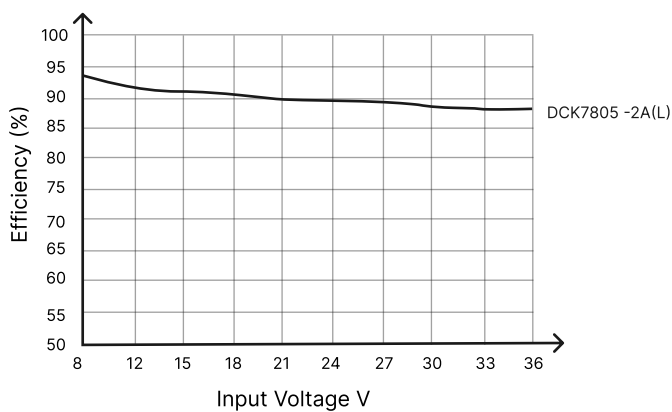
Figure 6: Efficiency Vs Input Voltage
