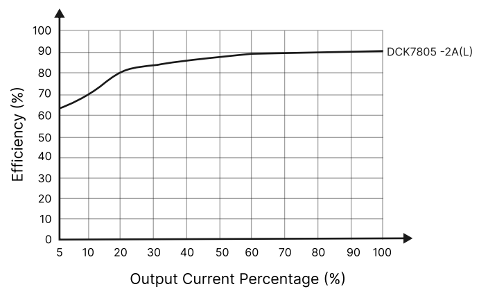
Figure 5: Efficiency Vs Output Load
