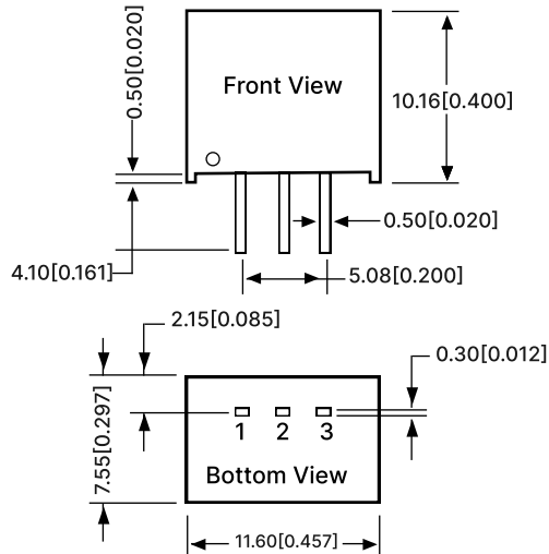
Figure 7: Overall dimensions
