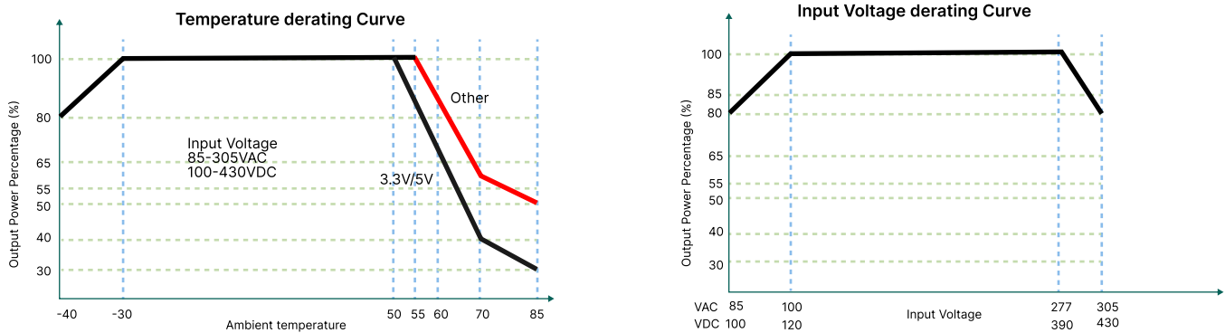
Figure 3: Voltage tolerance envelope
