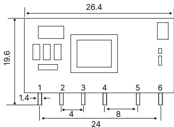
Figure 7: Overall dimensions
