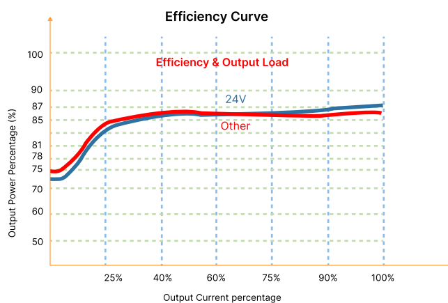
Figure 5: Efficiency VS Output Load (Nominal Voltage Input)
