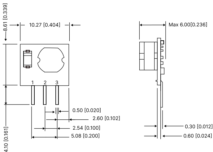
Figure 7 : Overall dimensions
