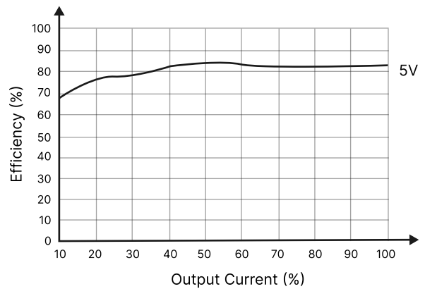
Figure 5: Efficiency Vs Output Load
