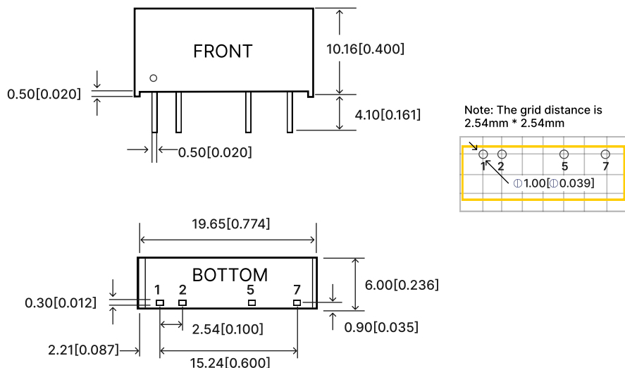
Figure 7: Overall dimensions
