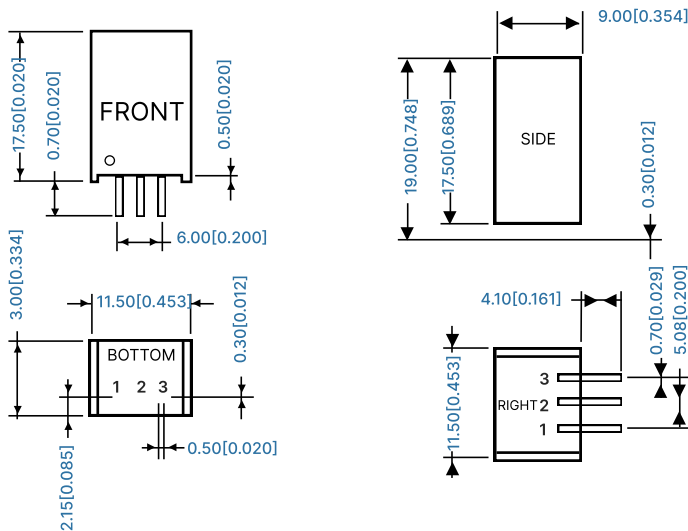
Figure 7: Overall dimensions
